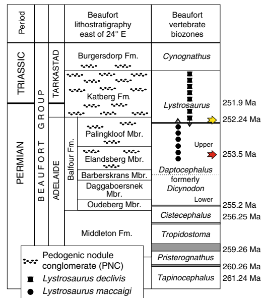
Fig. 1 Generalized stratigraphy of the Permian-Triassic Beaufort Group, Karoo Basin, South Africa, with vertebrate biozones. U-Pb age assignments separating the Tropidostoma , Cistecephalus , and Daptocephalus AZs from Day et al. 24 and Rubidge et al. 26 ; red arrow is lower Changhsingian age in the Elandsberg Member 20 ; yellow arrow is date reported, herein; and published postulated position of the Permian-Triassic boundary age (as based on the marine record 7 ). Vertebrate-range extensions follow re-analysis of original data 28 set used to interpret the terrestrial response to the end-Permian event 3,4 .
