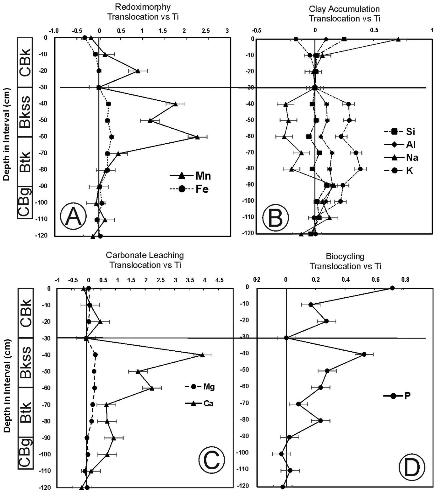
FIG. 10.—Mass-balance plots for redoximorphy, clay accumulation, carbonate leaching, and biocycling versus profile depth following Driese et al. (2000). Data were calculated against C horizons identified at depths of 30 cm and 110–120 cm. A) Translocation of Mn and Fe through the calcic Vertisol profile versus Ti as the immobile element. B) Translocation of Si (dashed line), Al (long dashed line), Na (solid line), and K (short dashed line) across the Vertisol profile using Ti as the immobile element. C) Translocation of Mg and Ca in the 1.3-m calcic Vertisol profile using Ti as the immobile element. D) Translocation of P in the calcic Vertisol profile using Ti as the immobile element.
