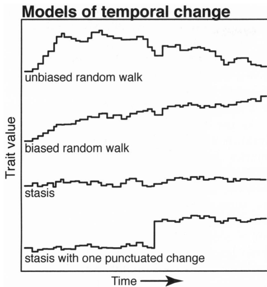
FIGURE 4. Examples of four alternative models of character change through time, with a hypothetical character (y-axis) plotted against time (x-axis). An unbiased random walk is equally likely to increase or decrease. A biased random walk tends to move in one direction over the alternative (illustrated here as a secular increase). Stasis tends to maintain a single mean value. Stasis with punctuated change is a model of stasis with two different mean values separated by a distinct transition. See Hunt (2006, 2008a,b) for more detailed explanations of the four models.
