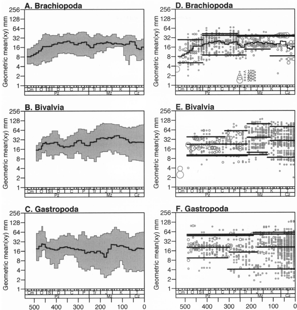
FIGURE 5. Occurrence-weighted shell size by taxonomic group. Phanerozoic timescale on the x-axis as in Figure 2. Geometric mean of x and y on the y -axis in millimeters with a \log_2 scale. In the left column (A–C), the solid black line is a three-point (three-bin) moving average of the mean occurrence-weighted shell size. The gray area is bounded by the 5th and 95th quantiles, which are used as proxies of the smallest and largest occurring shell sizes. In the right column (D–F) are the mean, 5th, and 95th quantiles as fit by PaleoTS (heavy black lines); each genus is plotted with a circle the size of which is proportional to its relative occurrence in the time bin. The three groups show distinct and independent histories of change in shell size.
