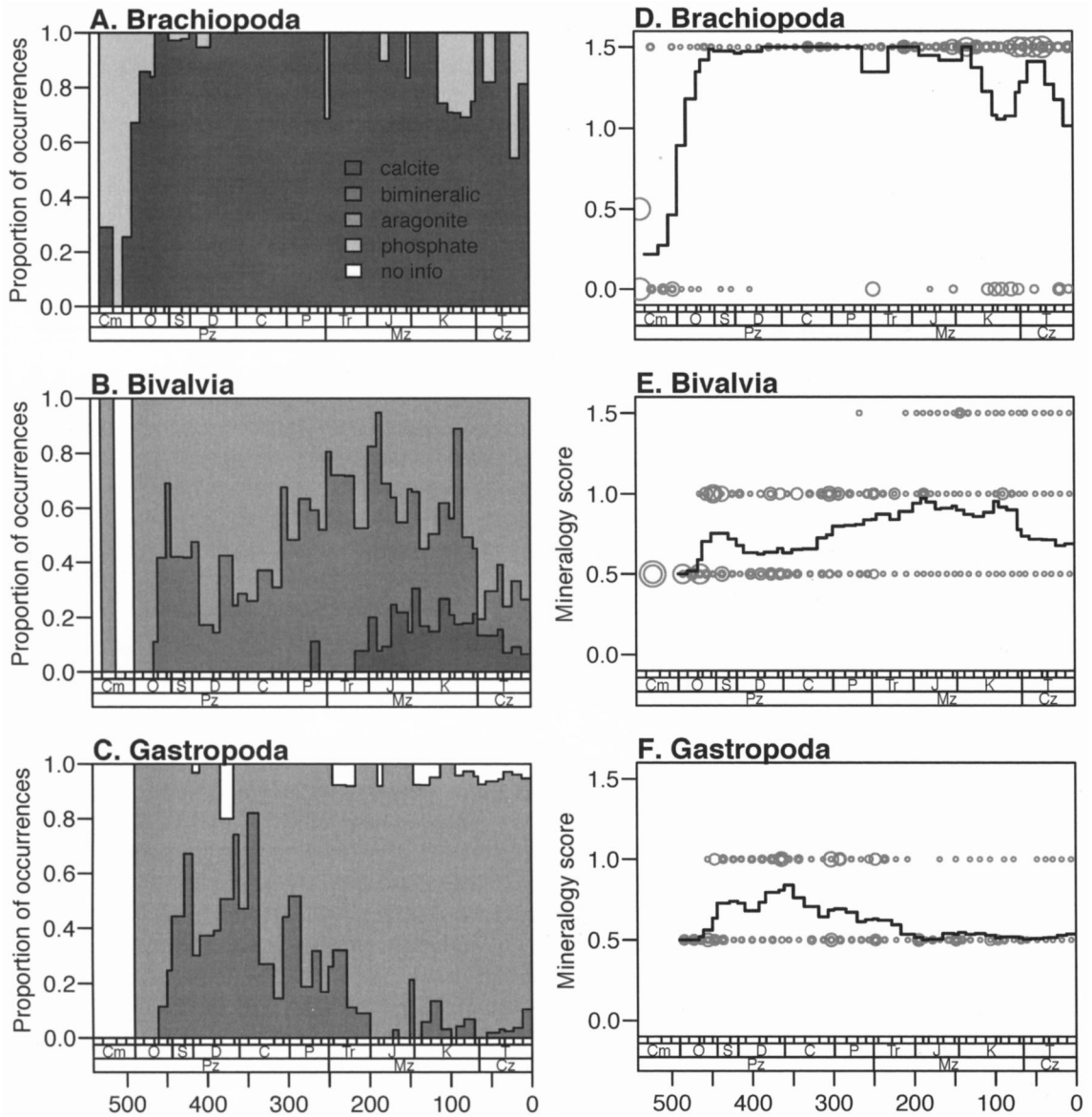
FIGURE 8. Occurrence-weighted shell mineralogy by taxonomic group. Format as in Figure 7. Mineralogy scores from least to most durable are 0 = organophosphatic, 0.5 = entirely aragonitic, 1.0 = bimineralic, 1.5 = entirely calcitic. Each group exhibits a different pattern of change in intrinsic durability, and peak durability (maximum calcitic genera) occurs at different times.
