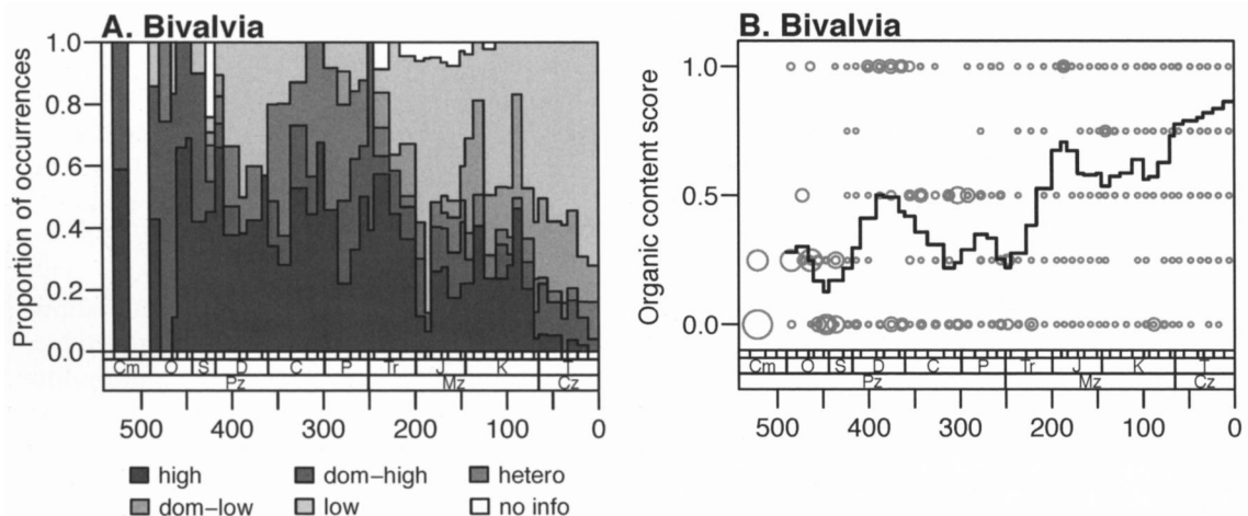
FIGURE 9. Occurrence-weighted shell organic content for bivalves. Format as in Figure 7. Organic content scores from least to most durable are 0 = high organic, 0.25 = dominantly high hetero-organic, 0.5 = hetero-organic, 0.75 = dominantly low hetero-organic, 1.0 = low organic. Genera having the most durable shells (composed entirely of low-organic-content microstructures) become increasingly abundant over time.
