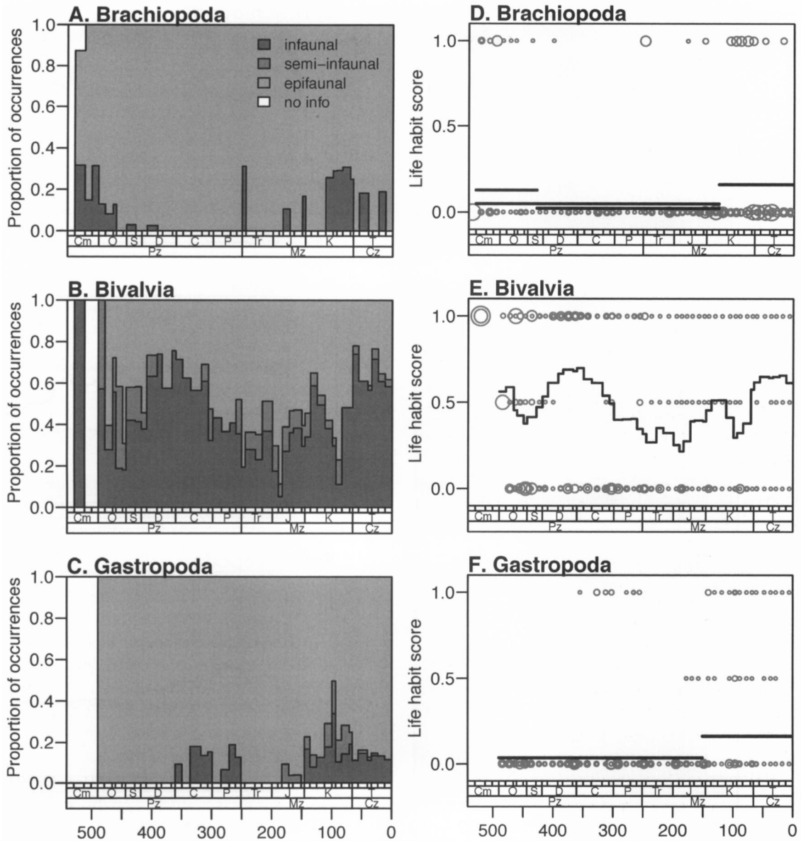
FIGURE 7. Occurrence-weighted life habit by taxonomic group. The left column (A–C) depicts the proportion of each bin’s occurrences represented by each life habit on the y-axis. The right column (D–F) shows the mean life-habit score as fit by PaleoTS (black line), with each genus plotted as a circle proportional to its relative occurrence in the time bin. Life-habit scores: 0 = epifaunal, 0.5 = semi-infaunal, 1 = infaunal. Each group exhibits a different pattern of change in intrinsic durability, and peak durability (maximum infaunality) occurs at different times.
