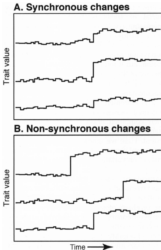
FIGURE 1. Examples of synchronous (A) and non-synchronous (B) changes through time in three different groups (e.g., brachiopods, bivalves, and gastropods over the Phanerozoic). Synchronous changes over time in the average durability of different groups suggests that they responded to the same extrinsic driver, which might be biological or taphonomic (e.g., a shared response to increased predation as a result of the Mesozoic Marine Revolution, to increased bioturbation and its cascading effects on dissolution, or to decreasing lithification and associated sieve effects). Non-synchronous changes in durability, denoting a different history for each group, indicate intrinsic causes (caused by macroevolution within each group).
