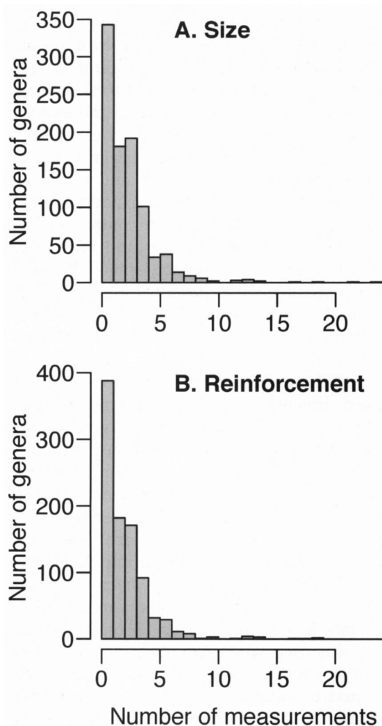
FIGURE 3. Histograms of the number of genera (y-axis) with a given number of specimens (x-axis) measured for shell size (A) and shell reinforcement (B). Approximately half of the genera in our durability data set are based on examination of two or more specimens.
