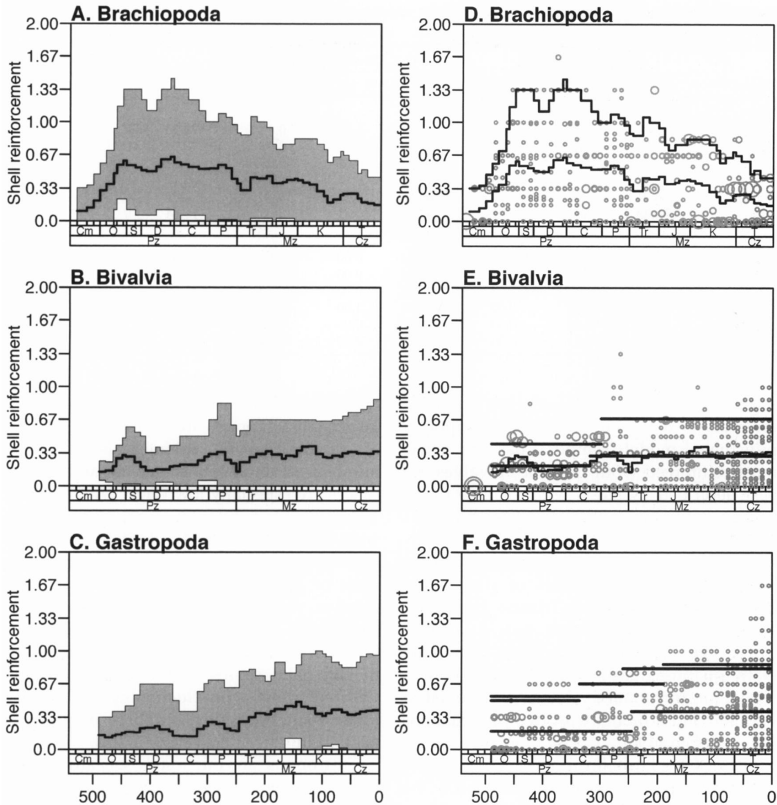
FIGURE 6. Occurrence-weighted shell reinforcement by taxonomic group. Shell reinforcement on the y-axis with an arithmetic scale; format otherwise as in Figure 5. Groups show distinct patterns of change, providing support for both random walk and punctuated models.
