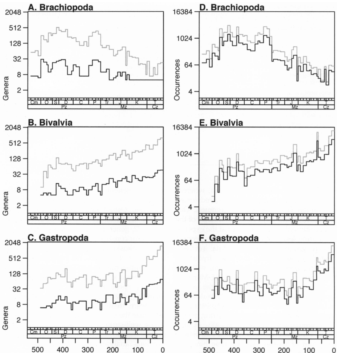
FIGURE 2. Change over the Phanerozoic in the number of genera (A–C, left column; log 2 ) and number of occurrences (D–F, right column; log 2 ) of the major taxonomic groups analyzed here, based on data from the Paleodb. Phanerozoic timescale on the x-axis with geologic age (Ma), eras, periods, and analytic time bins (~11 Myr each). Gray lines indicate the total numbers recorded in the Paleodb, and black lines indicate numbers for the most common 1002 genera analyzed here (occurrence data set).
