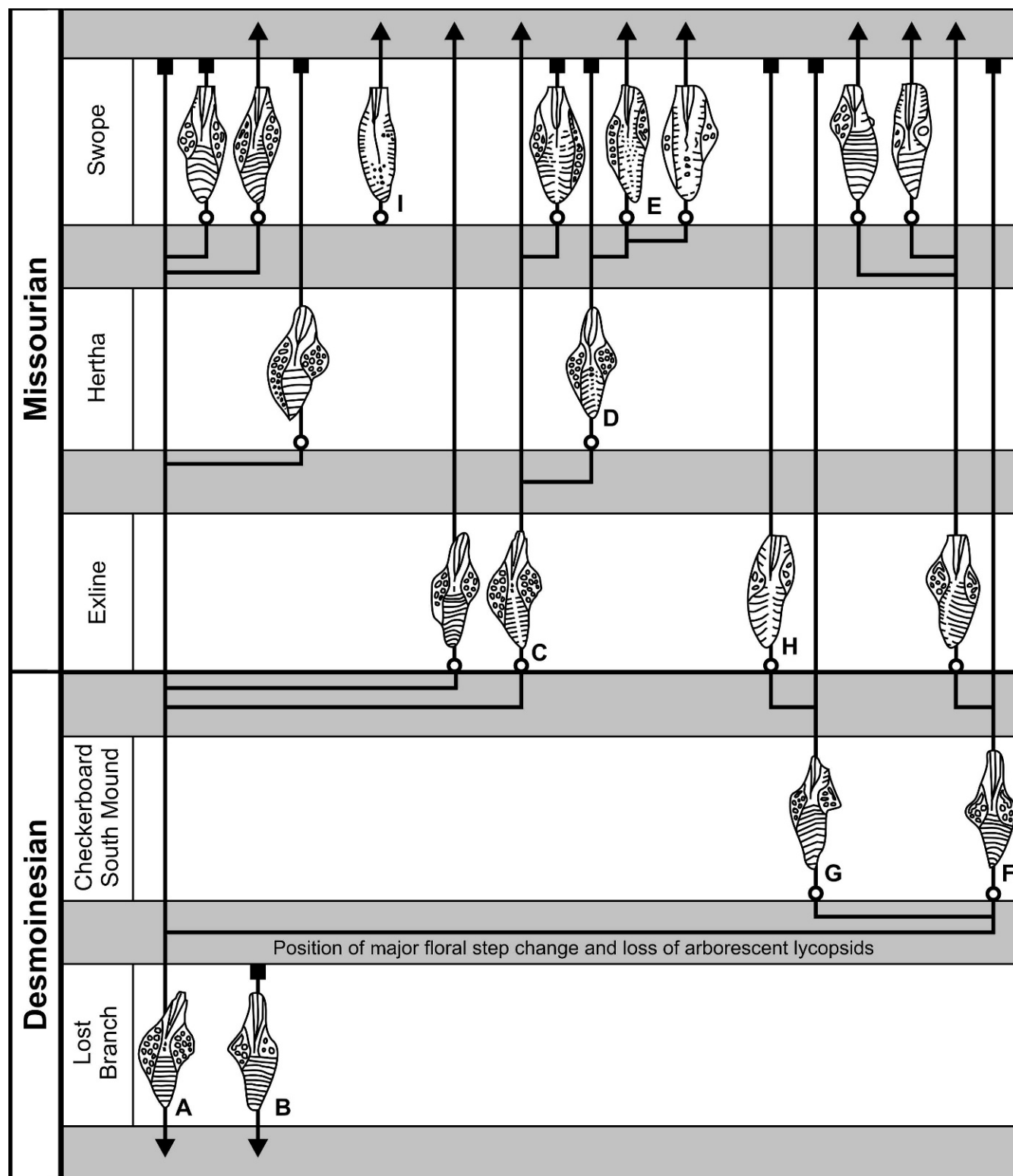
FIGURE 4— Idiognathodus diversification from Lost Branch to Swope cyclothem of the Midcontinent Basin (after Rosscoe, 2008; Rosscoe and Barrick, 2009b) within the Kasimovian Stage (spanning Desmoinesian–Missourian boundary). Gray = sequence boundaries separating cyclothem on mid shelf; thick black lines = species ranges, with arrows indicating continuation of range beyond chart; open circles = FAD; closed squares = LAD. Key taxa indicated by bold letters: A = I. swadei , B = I. expansus , C = Idiognathodus sp. Z, D = I. turbatus , E = I. cancellosus , F = I. sulciferus , G = I. harkeyi , H = I. eccentricus , I = I. biliratus .
