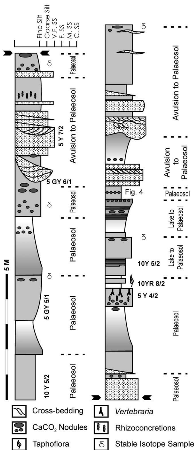
Fig. 3. Measured stratigraphic section along the R61 along side of which are interpreted depositional environments of each aggradational sequence. The plant-fossil assemblage preserved directly above a Vertebraria -rooted siltstone (palaeosol) is entombed in a yellow-white devitrified claystone. Additional floral elements also are preserved within a mixed siltstone and claystone lithology up to 40 cm above the contact with the palaeosol.
